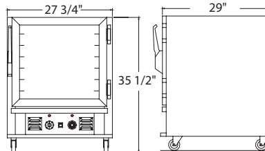
DP7D
