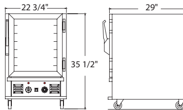
DP7D
